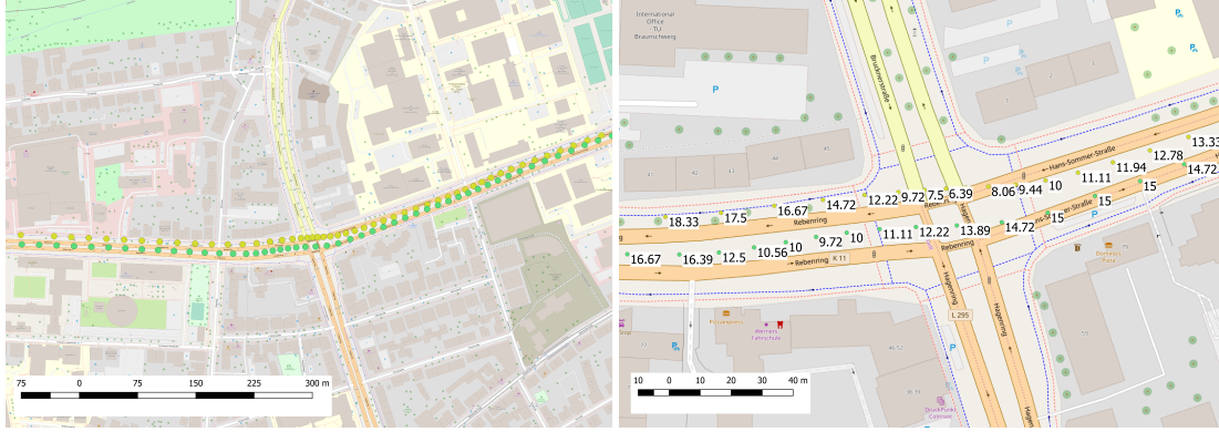
(a) Test intersection Rebenring / Hagenring in Braunschweig with recorded positions of two emergency vehicles. (b) Detail view of the test intersection. The annotations at the points correspond to the momentary speed of the test vehicles.
